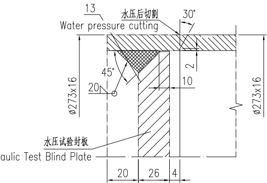
集箱进出口详图 Detailed Drawing of Inlet/Outlet for Steam Header 1:4
