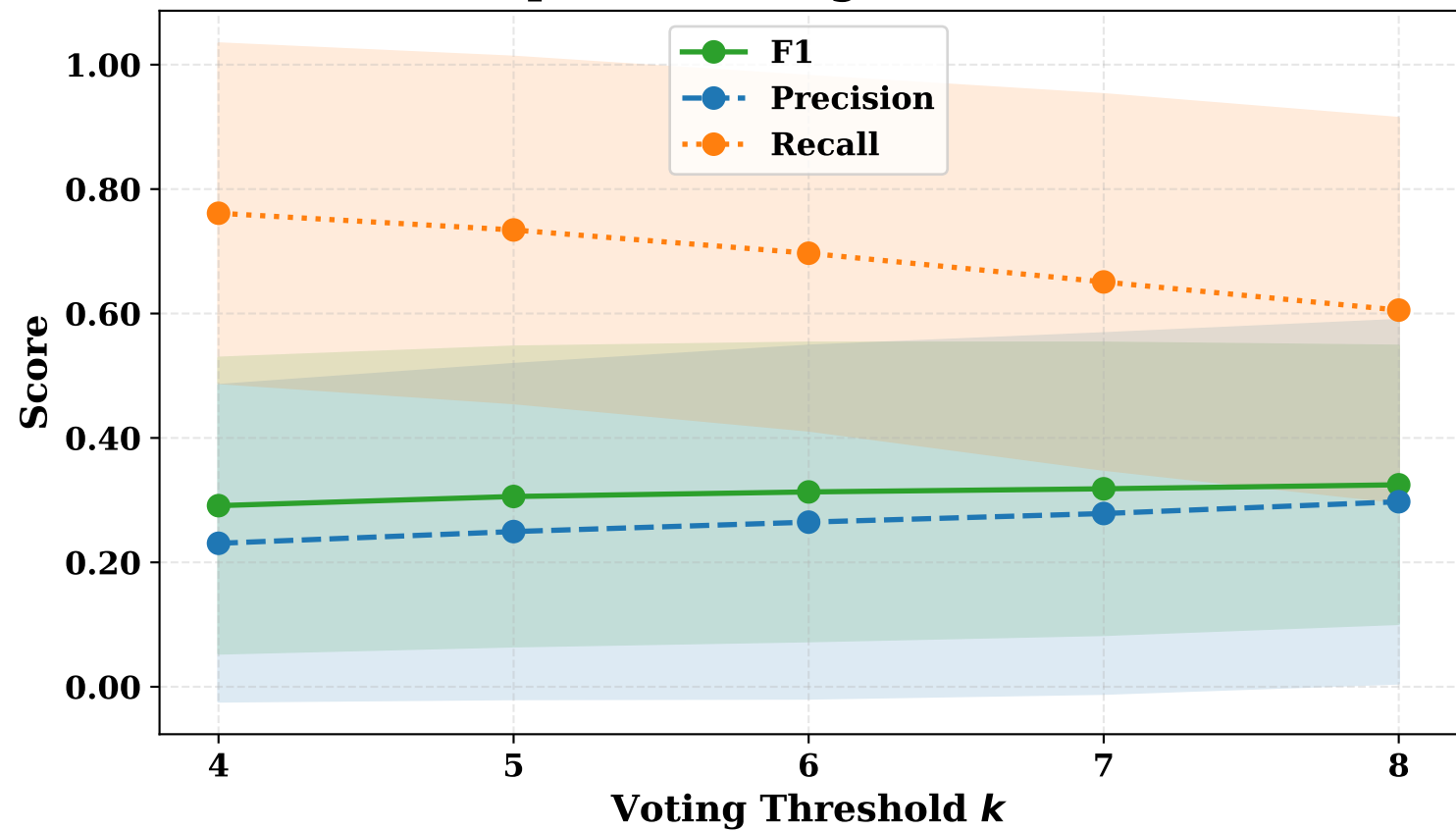
Impact of Voting Threshold k
