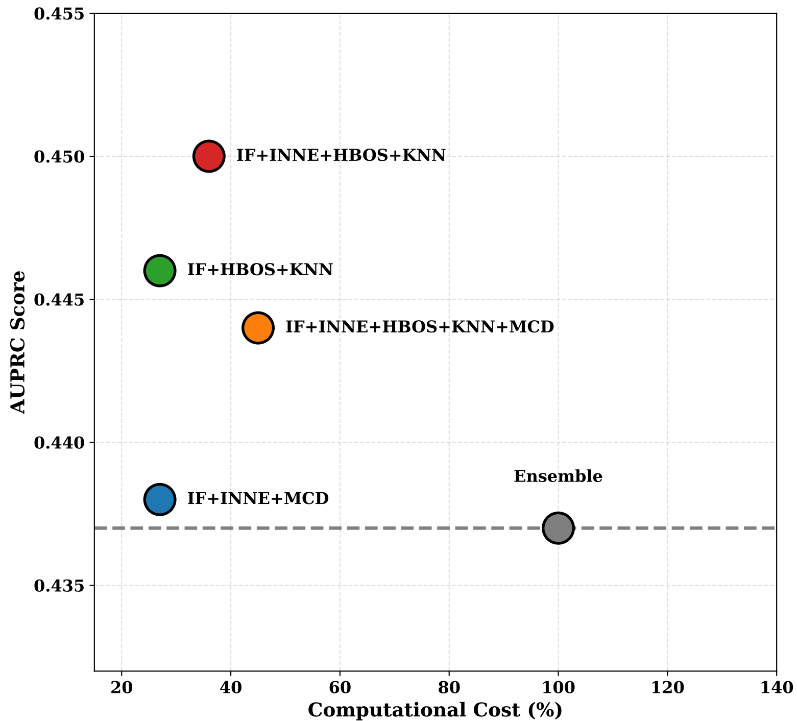
AUPRC Score vs Cost
