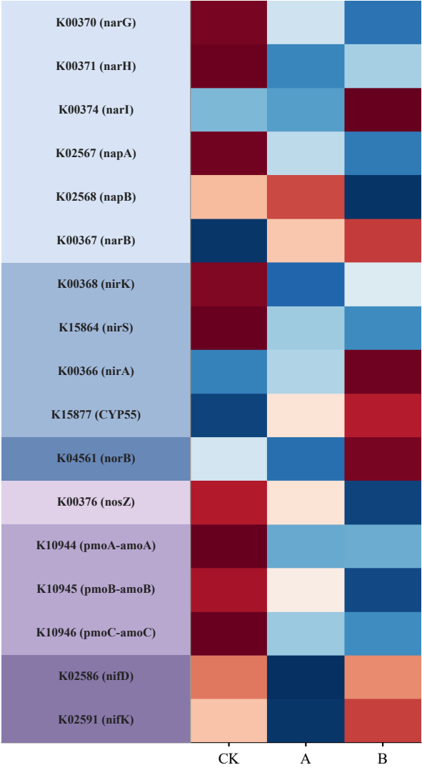
(c) 氮代谢
