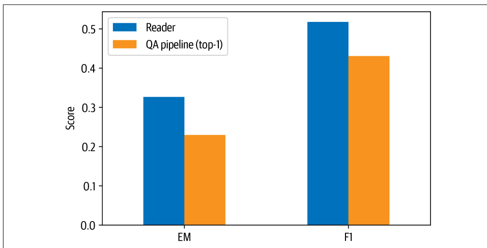
Figure 7-12. Comparison of EM and F_1 scores for the reader against the whole QA pipeline
