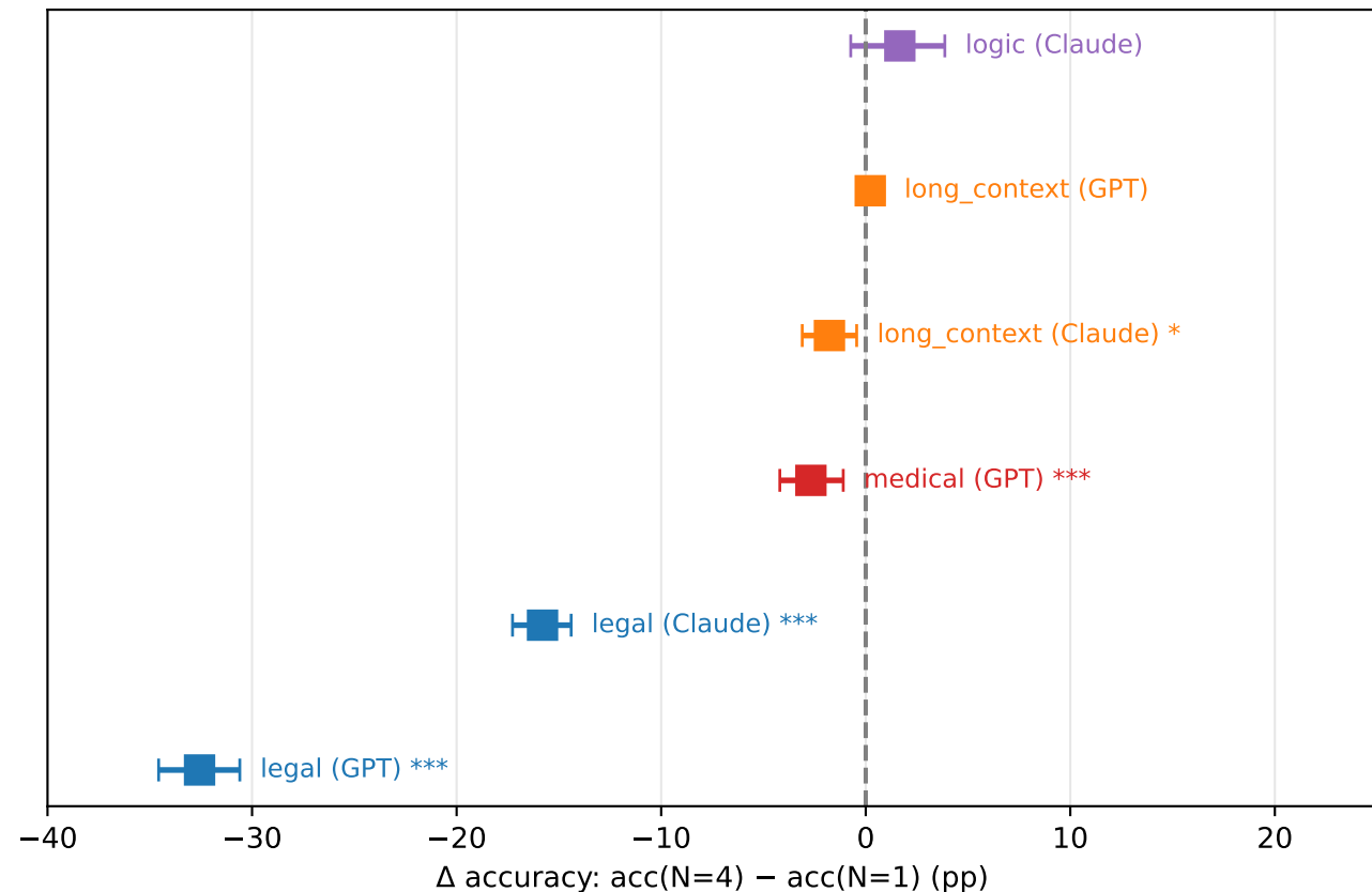
(b) N=1 vs N=4 paired comparison (McNemar significance: ***p<0.001, **p<0.01, *p<0.05)
