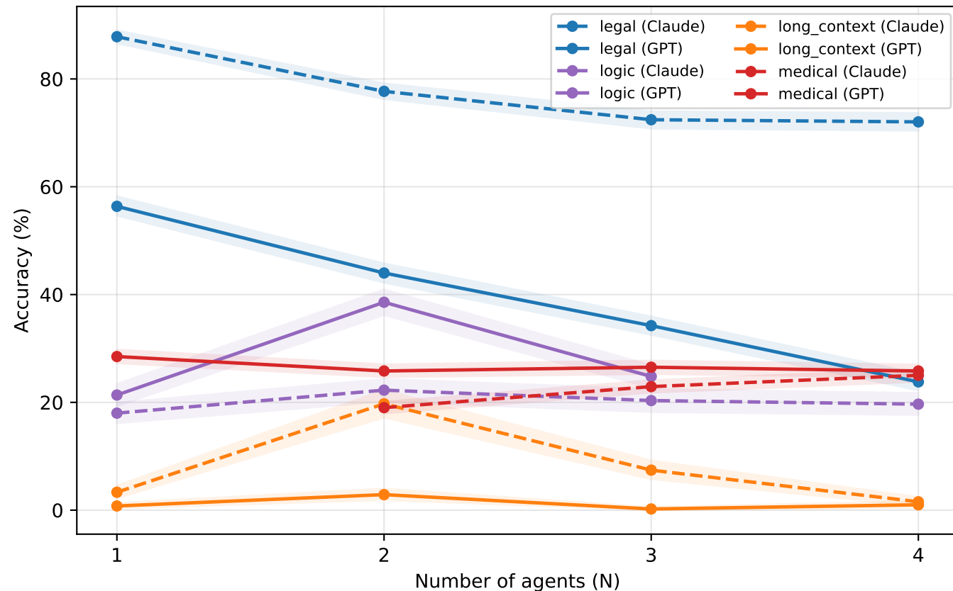
(a) Per-cell accuracy with 95% bootstrap CI
