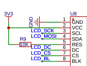
LCD Screen
