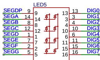
LED Matrix
