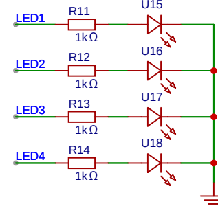
LED Matrix
