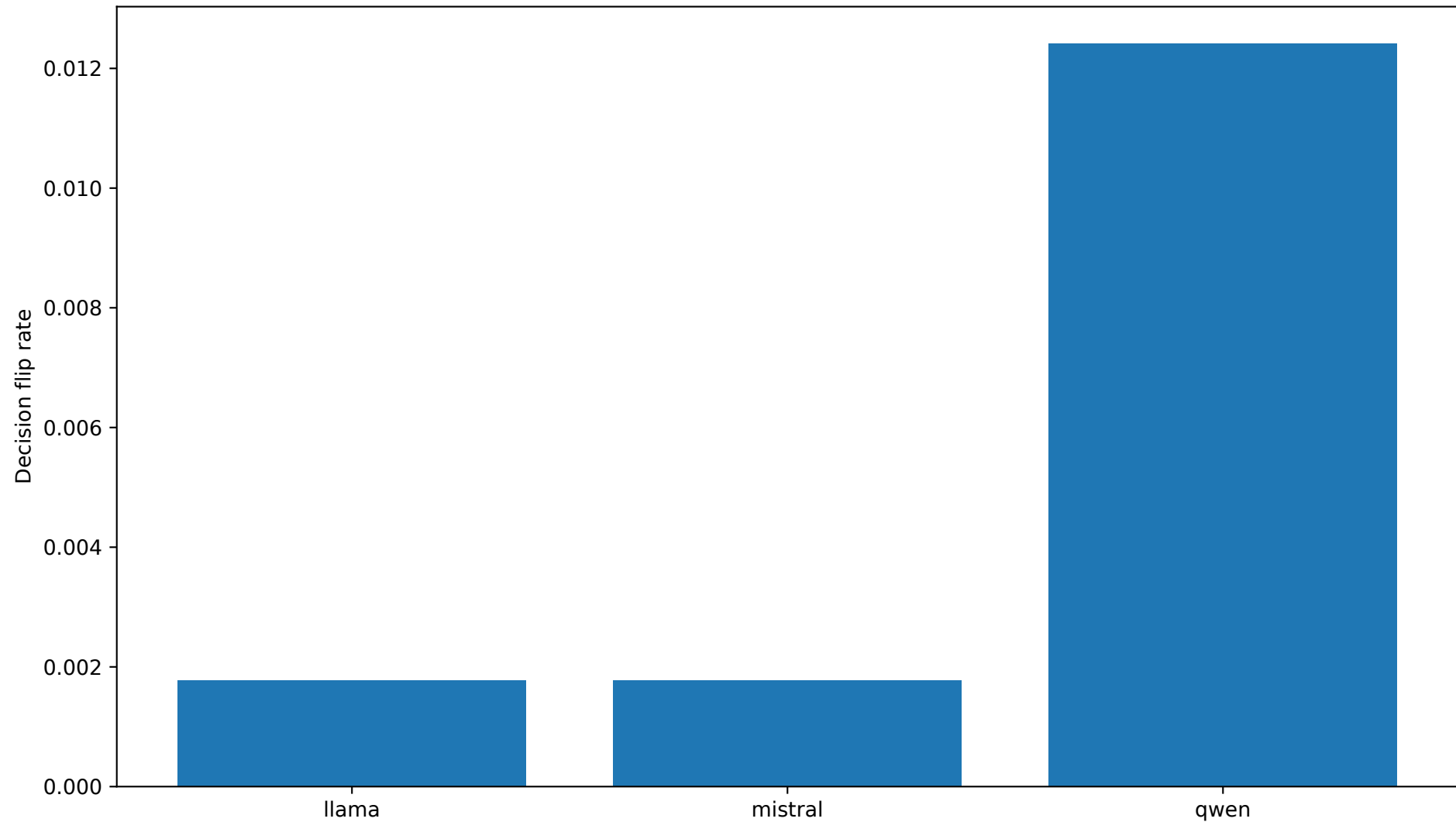
Decision flip rate by model
