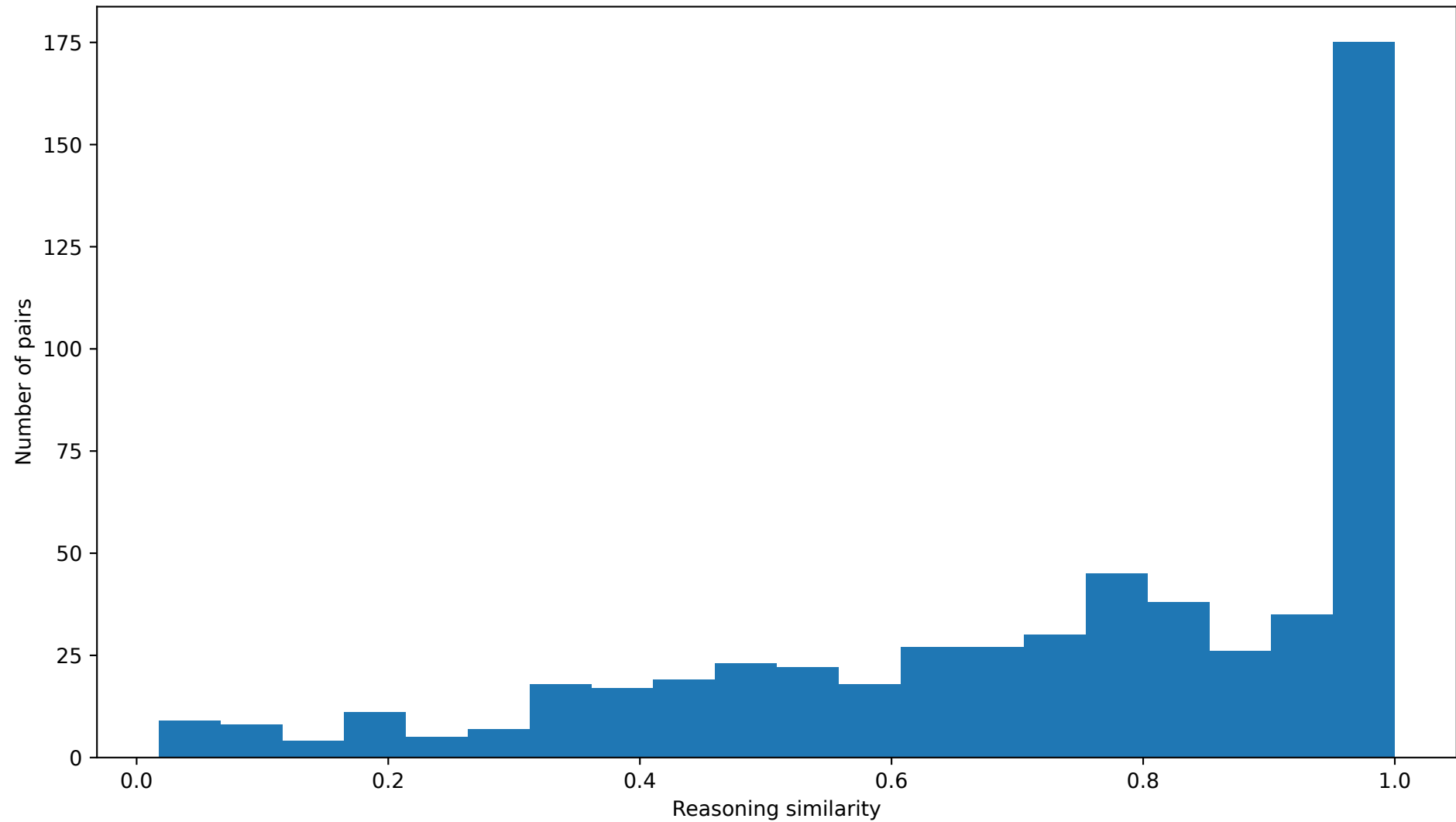
Reasoning similarity distribution - llama
