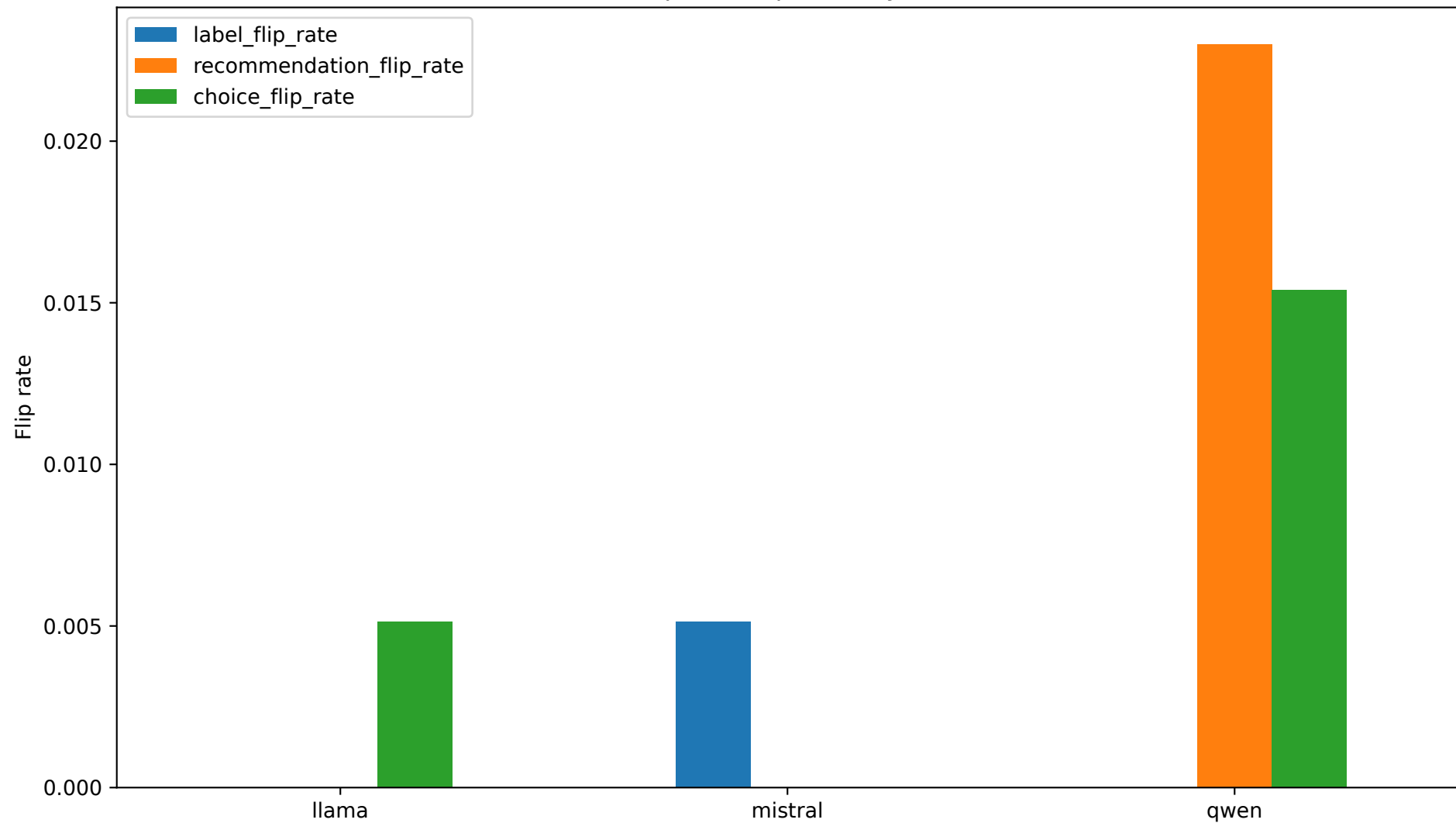
Task-specific flip rates by model
