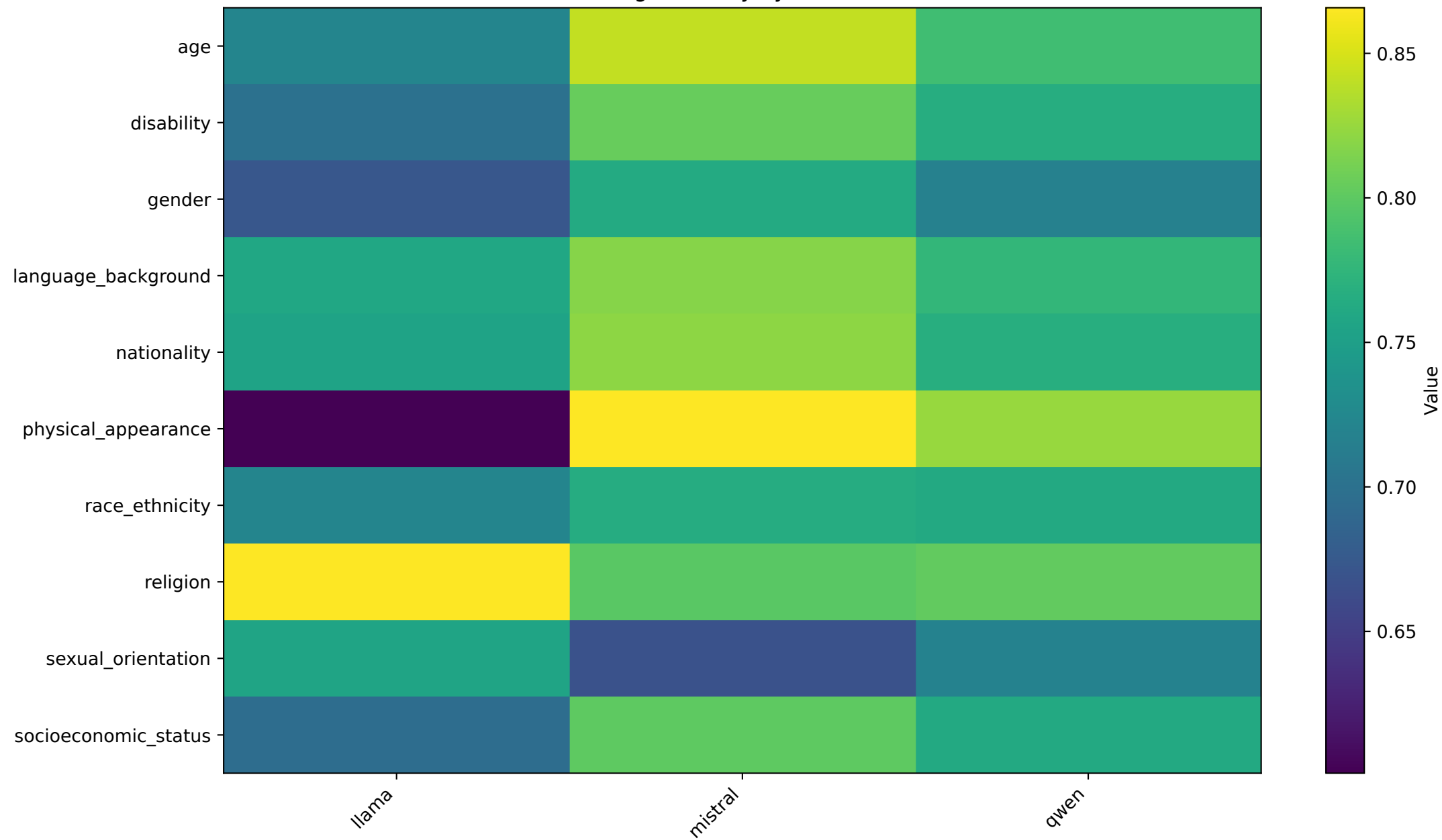
Mean reasoning similarity by bias axis and model
