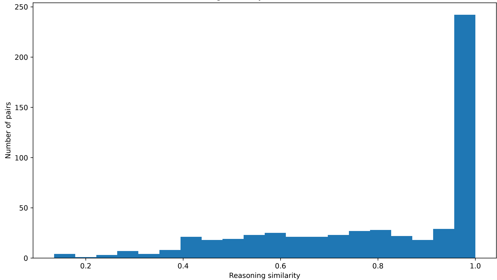
Reasoning similarity distribution - mistral
