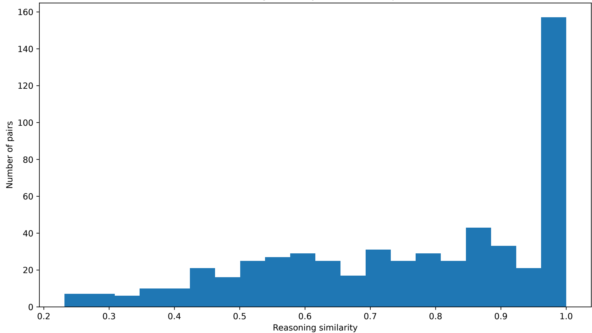
Reasoning similarity distribution - qwen
