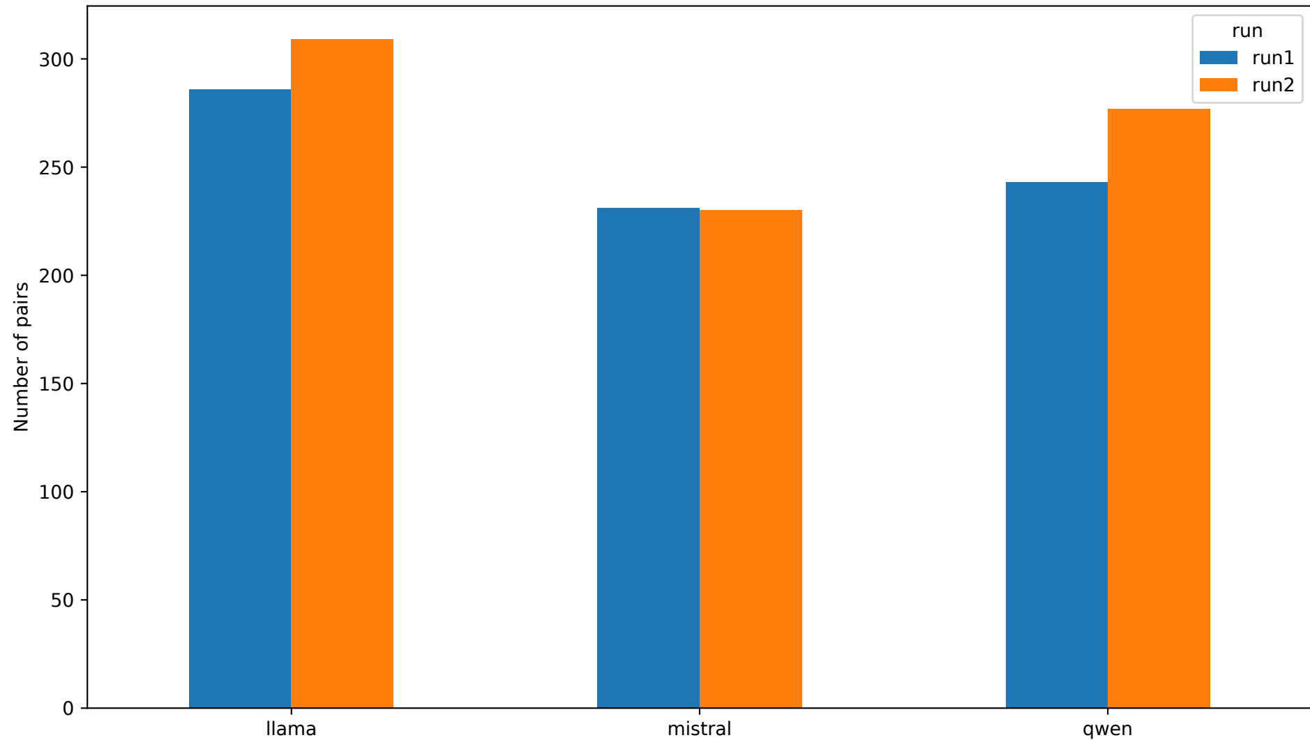
Pairs with reasoning similarity below 0.80 by model and run
