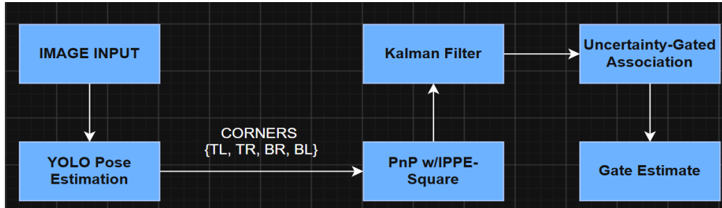
Fig. 6. Conceptual diagram of the perception pipeline during inference.
