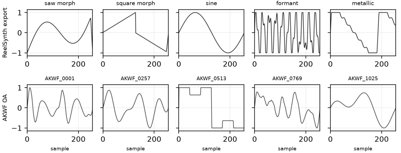
Figure 18: Compact wavetable diversity gallery from existing exports (one mid-morph dry frame per unique ReelSynth factory bank, top; matched AKWF CC0 cycles, bottom). No new NAS for this panel. Quantitative wrap scores: Table 10.
