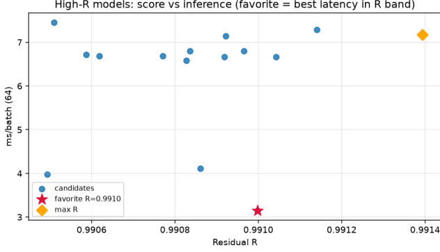
Figure 12: High- R fitted operators: residual vs CUDA latency. Star: favorite.
