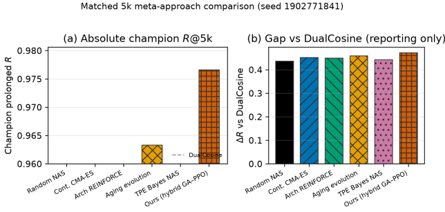
Figure 21: Matched 5,000-evaluation search methods under locked R_{\text{blend}}+J (seed 1902771841). Table 18 reports mean \pm std across three search seeds. Dashed line: Dual Cosine on the same runner.
