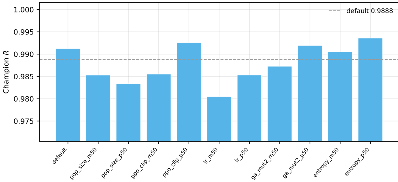
HP sensitivity (matched budget arms)
