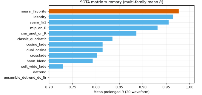
Figure 8: Multi-family mean prolonged R by method (same 20-waveform board as Table 7).
