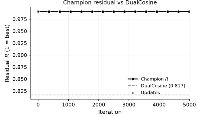
Figure 18: 5k-gate search freeze: champion residual R versus clean search iteration (x-axis capped at 5,000), with DualCosine baseline on the runner geometry (RTX 3090). Accessibility: black line with circle markers; DualCosine as a dashed gray baseline.
