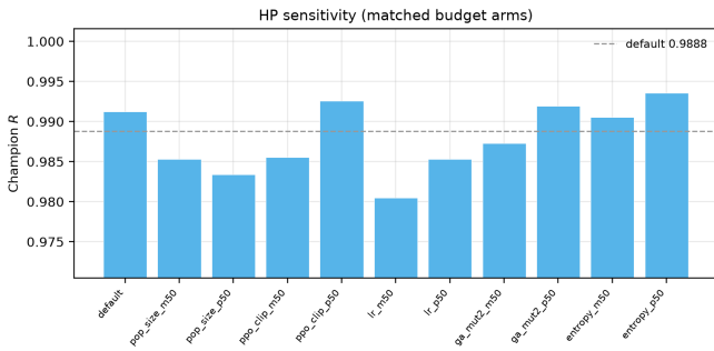
Figure 28: One-at-a-time \pm 50\% hyperparameter sensitivity of hybrid champion R at a 500-iteration budget (seed 1902771841). Blue bar / dashed line: Table 2 default. This is a sensitivity probe , not a full 5k re-search per HP.
