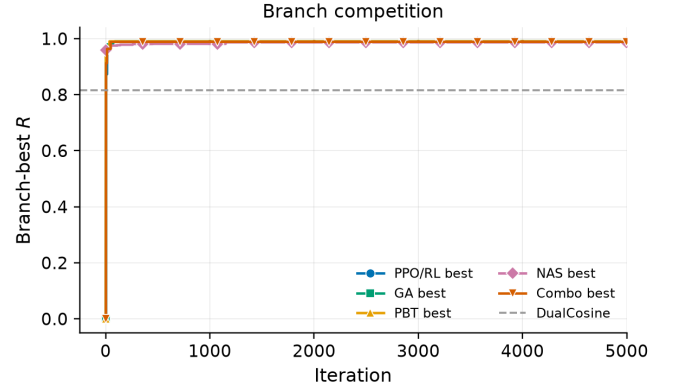
Figure 19: 5k-gate search freeze: per-branch best residual trajectories (PPO/RL, GA, PBT, NAS, combo) versus iteration (x-axis capped at 5,000). Accessibility: colorblind-safe colors plus distinct markers (circle, square, triangle, diamond, inverted triangle) for grayscale print.
