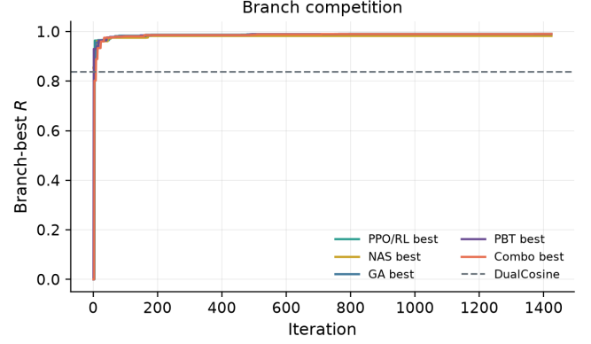
Figure 6: Interim per-branch best residual trajectories (PPO/RL, GA, PBT, NAS, combo). Monitoring only.
