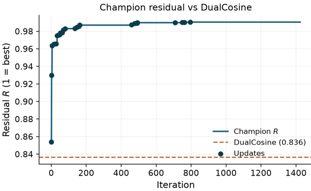
Figure 5: Interim champion residual R versus search iteration, with DualCosine baseline. Monitoring snapshot; not a final result.
