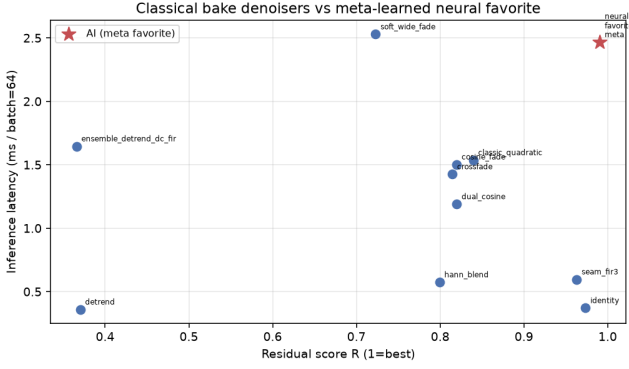
Figure 3: Classical bake denoisers vs neural favorite: residual R versus CUDA latency (ms/batch). Red star: AI favorite.
