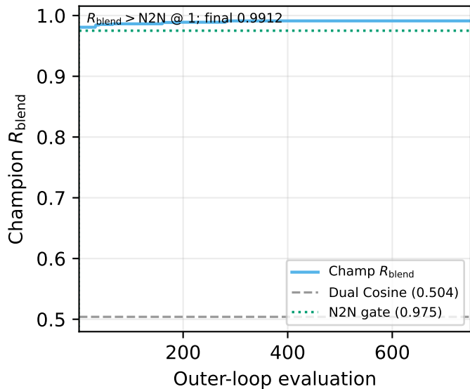
FitCell-to-plateau hybrid (750 evals)
