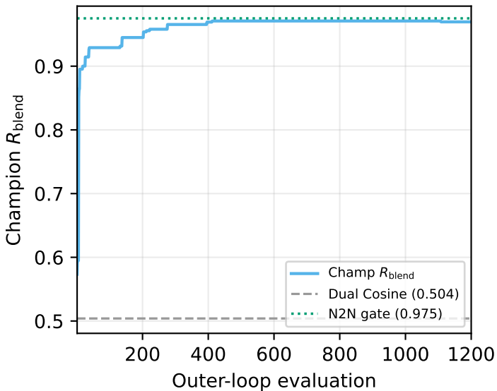
Short FitCell hybrid (1,200 evals)
