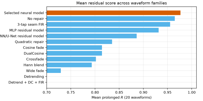
Figure 7: Multi-family mean prolonged R by method (same 20-waveform board as Table 7).
