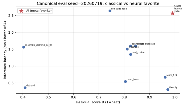
Figure 15: Canonical holdout (seed 20260719, batch 64): classical bake methods and neural favorite in the R vs CUDA ms/batch plane. Star: favorite.
