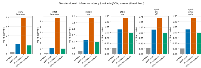
Figure 26: Transfer-domain inference latency (ms/batch). N2N is wavetable-trained zero-shot when available.
