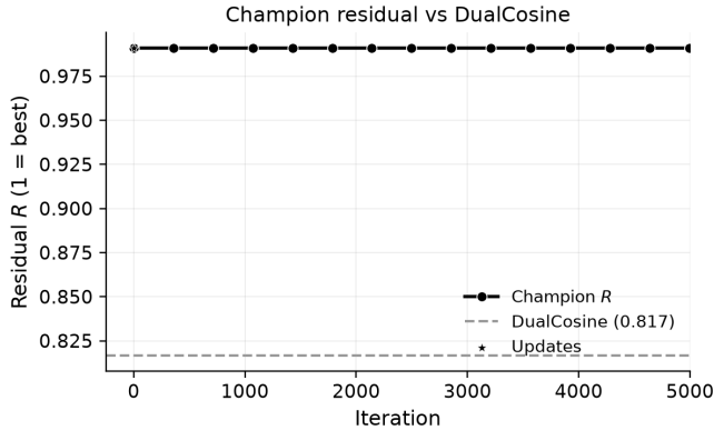
Figure 17: Champion residual R over the first 5,000 search iterations, with the DualCosine reference on the same runner geometry (RTX 3090). The black line uses circle markers; the reference is dashed gray.
