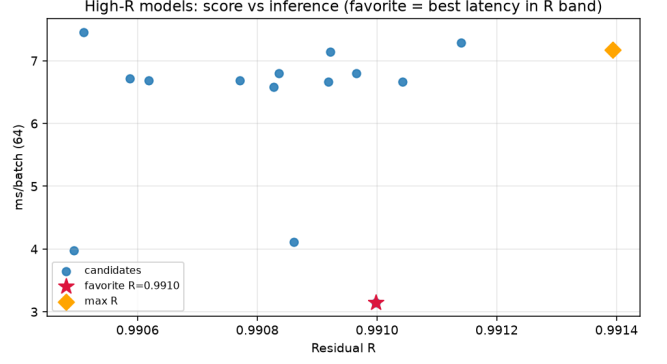
Figure 13: High- R fitted cells on CUDA (batch 64): prolonged residual R versus forward latency (ms/batch). Star marks the favorite (fastest inside the near-max- R band).
