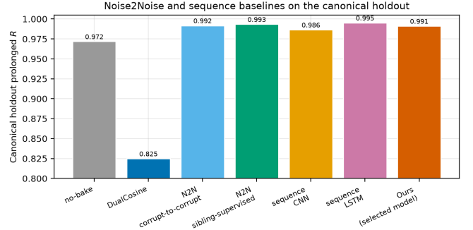
Figure 8: Canonical holdout prolonged R : N2N and seq baselines vs Ours (neural favorite). Train seeds 424242/424243 are disjoint from holdout 20260719.
