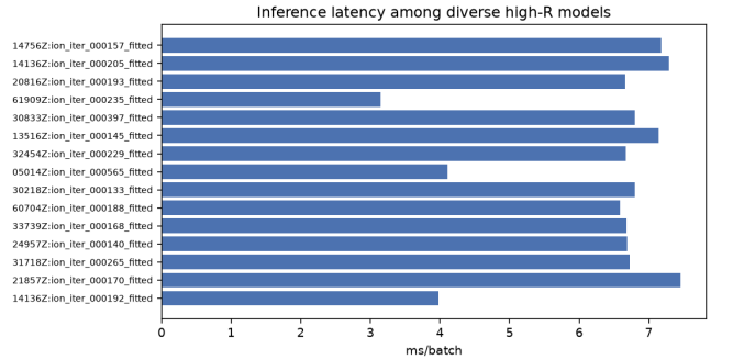
Figure 14: Inference latency (ms/batch, CUDA, batch 64) for diverse high- R fitted models from the inference bench.
