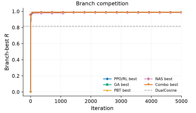
Figure 18: Best residual score reached by each search branch over the first 5,000 iterations (PPO/RL, GA, PBT, NAS, and combined). Colors and markers remain distinguishable in grayscale.
