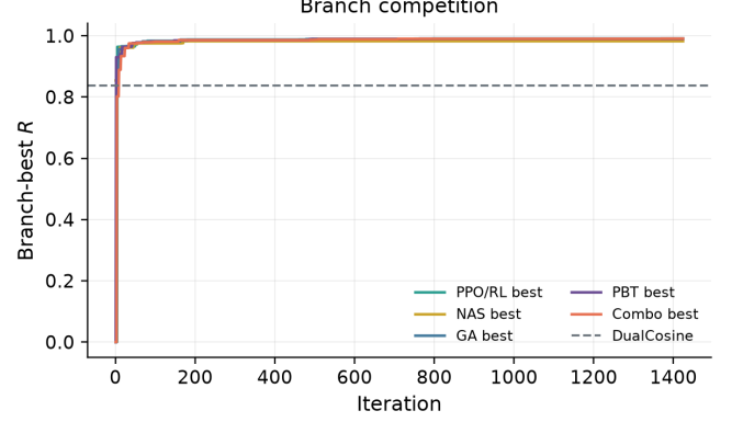
Figure 4: Interim per-branch best residual trajectories (PPO/RL, GA, PBT, NAS, combo). Monitoring only.
