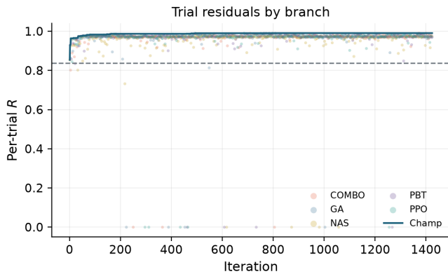
Figure 6: Interim per-trial residual scatter by search branch, with champion overlay. Monitoring snapshot.
