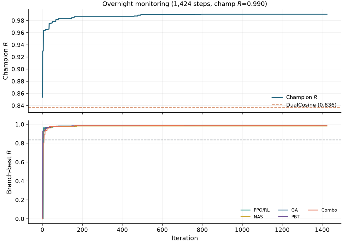
Figure 5: Full-width interim overnight monitoring panel: champion R (top) and branch-best trajectories (bottom). Snapshot while the GPU budget completes.
