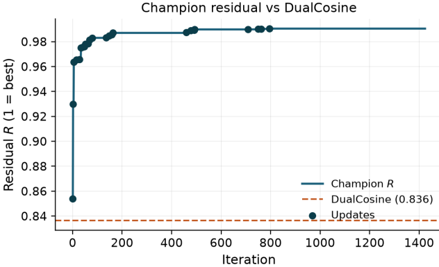
Figure 3: Interim champion residual R versus search iteration, with DualCosine baseline. Monitoring snapshot; not a final result.
