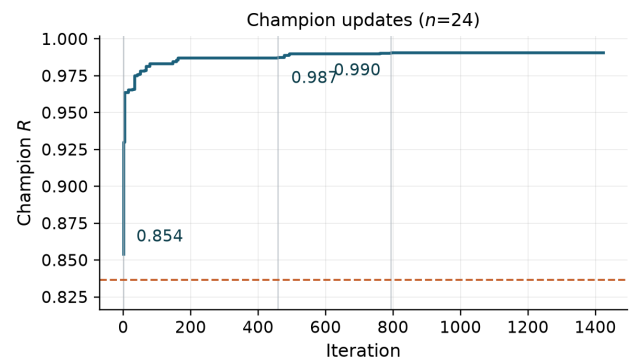
Figure 7: Interim champion update timeline. Sparse R labels mark first, peak-mid, and latest improvements to stay legible in twocolumn.
