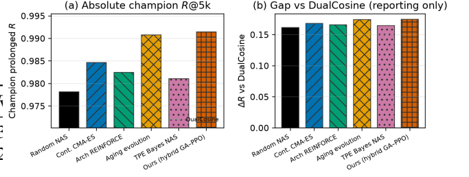
Figure 6: Matched 5k-budget meta-approach comparison (search seed 1902771841): (a) champion prolonged R ; (b) \Delta R vs DualCosine (reporting gap only; objective is maximize absolute R toward the ideal sibling). Manuscript names; Okabe-Ito colors with distinct hatches for grayscale print.
