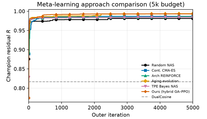
Figure 7: Matched 5k-budget meta-learning comparison: champion residual R versus outer iteration (x-axis capped at 5,000). DualCosine dashed as one classical comparator only. Objective is maximize absolute R toward the ideal sibling; rank vs the classical board in Table 4. Accessibility: Okabe-Ito colors with distinct markers for grayscale print.
