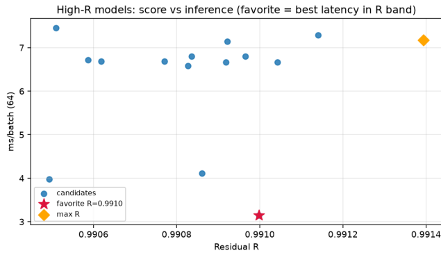
Figure 9: High- R fitted cells on CUDA (batch 64): prolonged residual R versus forward latency (ms/batch). Star marks the favorite (fastest inside the near-max- R band).
