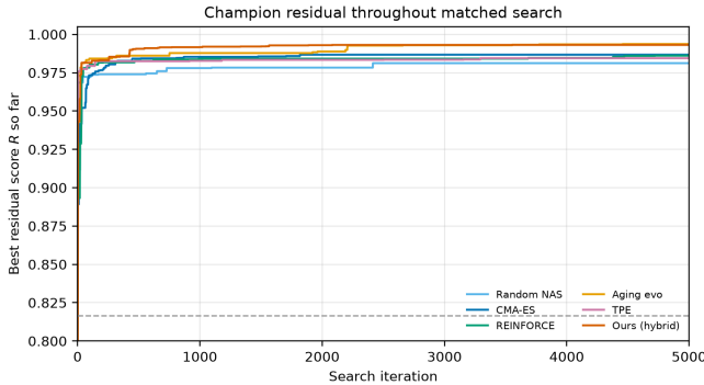
Figure 20: Champion residual R over a matched 5,000-evaluation budget. Dashed line: Dual Cosine.
