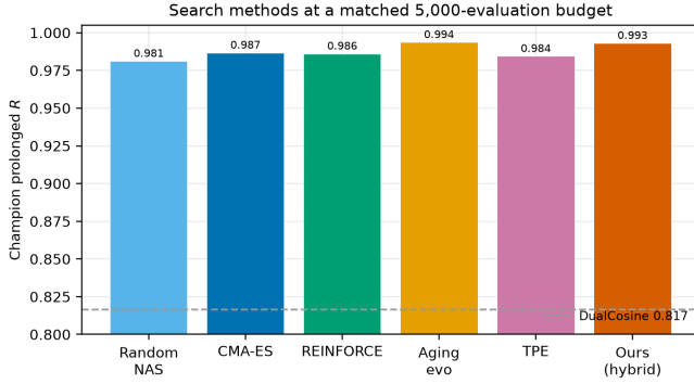
Figure 19: Matched 5,000-evaluation search methods (seed 1902771841). Champion prolonged R ; dashed line is Dual Cosine.
