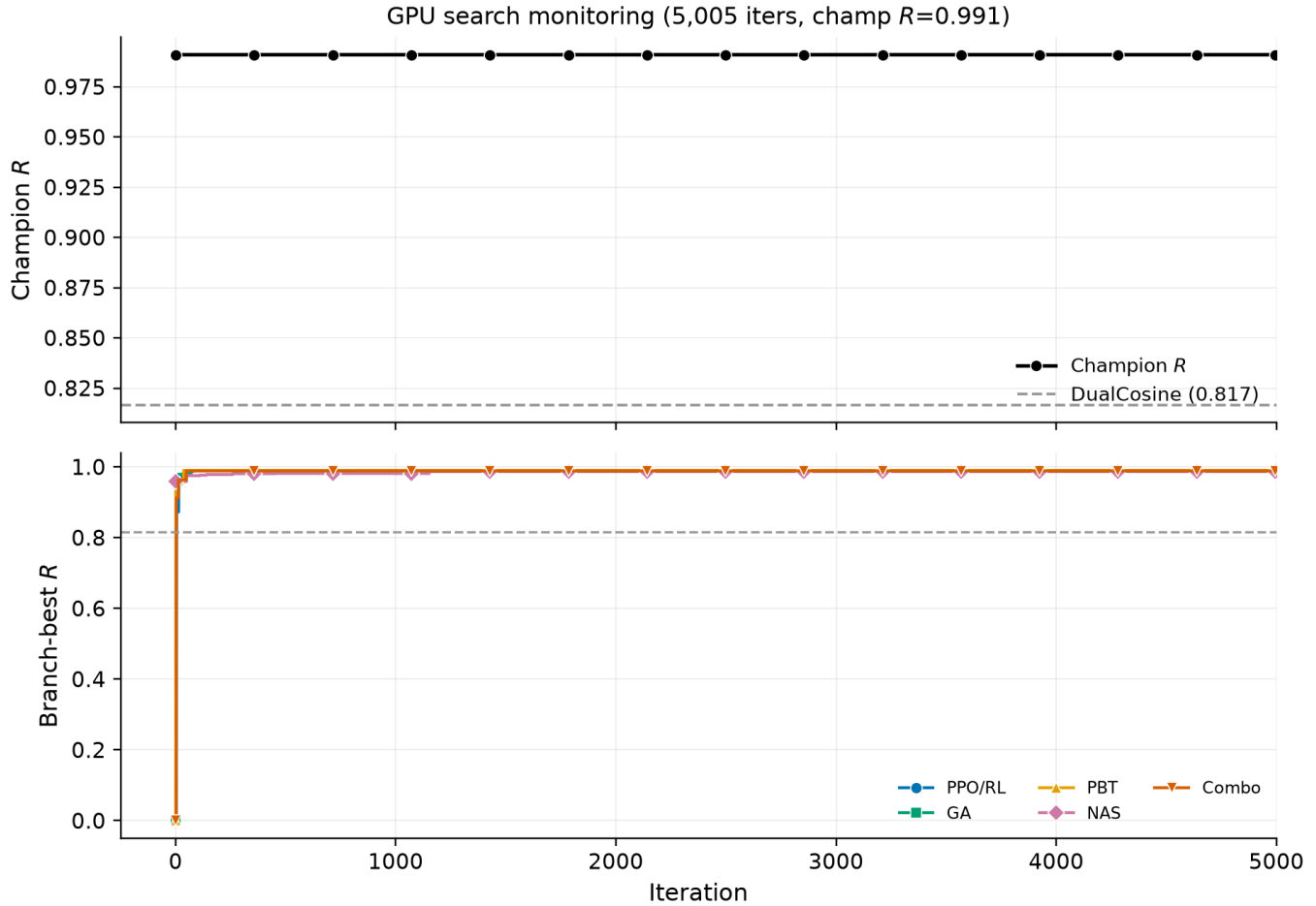
Figure 13: Full-width search monitoring panel at the 5k-gate freeze (first 5,000 iterations): champion R (top) and branch-best trajectories (bottom). Markers and Okabe-Ito colors match Figure 12. Source: history.jsonl .
