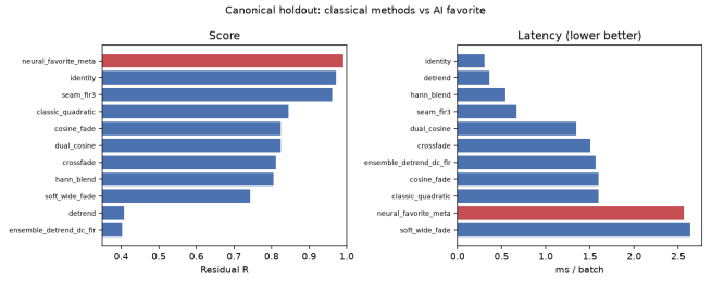
Figure 10: Canonical holdout ranking on prolonged residual R (left) and CUDA latency (right). DualCosine R \approx 0.825 . Favorite highlighted.
