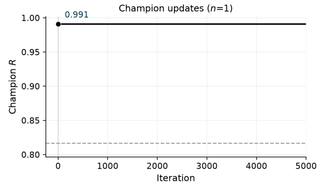
Figure 15: Champion update timeline for the first 5,000 iterations at the 5k-gate freeze. Sparse R labels mark first, mid-peak, and latest improvements for twocolumn legibility.
