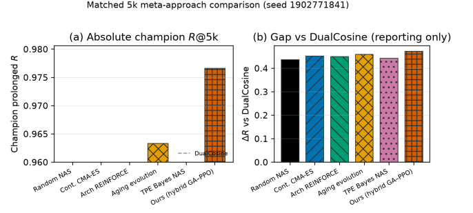
Figure 21: Matched 5,000-evaluation search methods under locked R_{\text{blend}}+J (seed 1902771841). Table 19 reports mean \pm std across three search seeds. Dashed line: Dual Cosine on the same runner.
