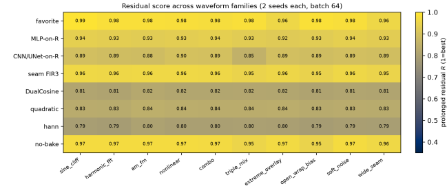
Figure 8: Colorblind-safe (cividis) heatmap of mean prolonged R for selected methods \times generative families (2 seeds each). Higher is better.
