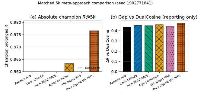
Figure 21: Matched 5,000-evaluation search methods under locked R_{\text{blend}} + J (seed 1902771841). Table 18 reports mean \pm std across three search seeds. Dashed line: Dual Cosine on the same runner.
