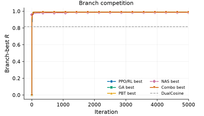
Figure 12: 5k-gate search freeze: per-branch best residual trajectories (PPO/RL, GA, PBT, NAS, combo) versus iteration (x-axis capped at 5,000). Accessibility: colorblind-safe colors plus distinct markers (circle, square, triangle, diamond, inverted triangle) for grayscale print.
