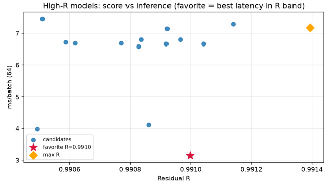
Figure 7: High- R fitted cells on CUDA (batch 64): prolonged residual R versus forward latency (ms/batch). Star marks the favorite (fastest inside the near-max- R band).
