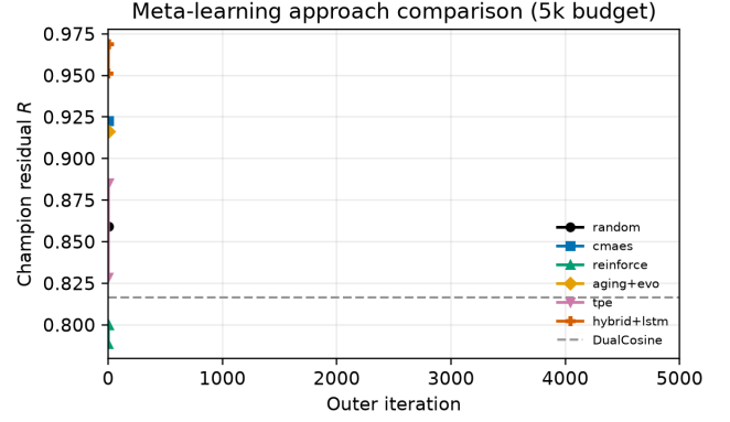
Figure 6: Matched 5k-budget meta-learning comparison: champion residual R versus outer iteration (x-axis capped at 5,000), including hybrid+LSTM. Accessibility: Okabe-Ito colors with distinct markers for grayscale print; DualCosine as a dashed gray baseline.
