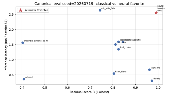
Figure 14: Canonical holdout: classical methods and favorite in the R vs ms/batch plane.
