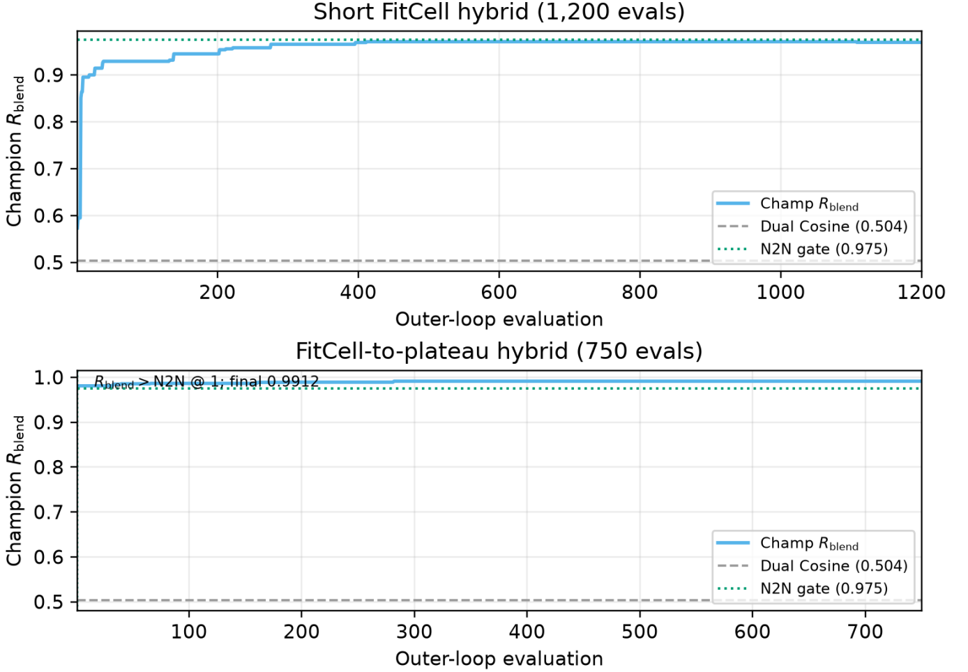
Figure 9: Hybrid search learning curves under R_{\text{blend}} (seed 1902771841). Top: short FitCell (1,200 evaluations; champ. \approx 0.9695 ). Bottom: FitCell-to-plateau (750 evaluations; champ. \approx 0.9912 ).
