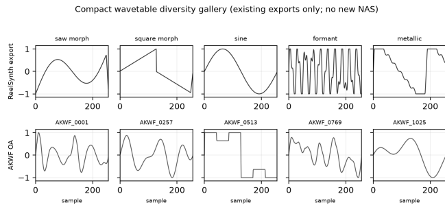
Figure 18: Compact wavetable diversity gallery from existing exports (one mid-morph dry frame per unique ReelSynth factory bank, top, and matched AKWF CC0 cycles, bottom). No new NAS for this panel. Quantitative wrap scores: Table 11.
