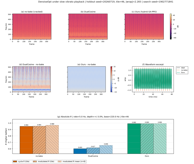
Figure 16: Slow-vibrato spectrogram eval on a high-wrap holdout tile (seed 20260719). (a–c) Magnitude spectrograms for no-bake, DualCosine, and Ours. (d–e) Spectrogram differences vs no-bake. (f) Short waveform excerpt. (g) Absolute R : cycle-local prolonged residual, modulated-playback residual on the same tile, and mean modulated R over top-wrap tiles. Accessibility: Okabe–Ito hues. Difference maps use diverging coolwarm. Formal human A/B scores are out of scope.
