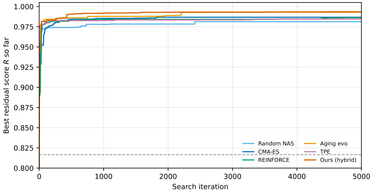
Champion residual throughout matched search
