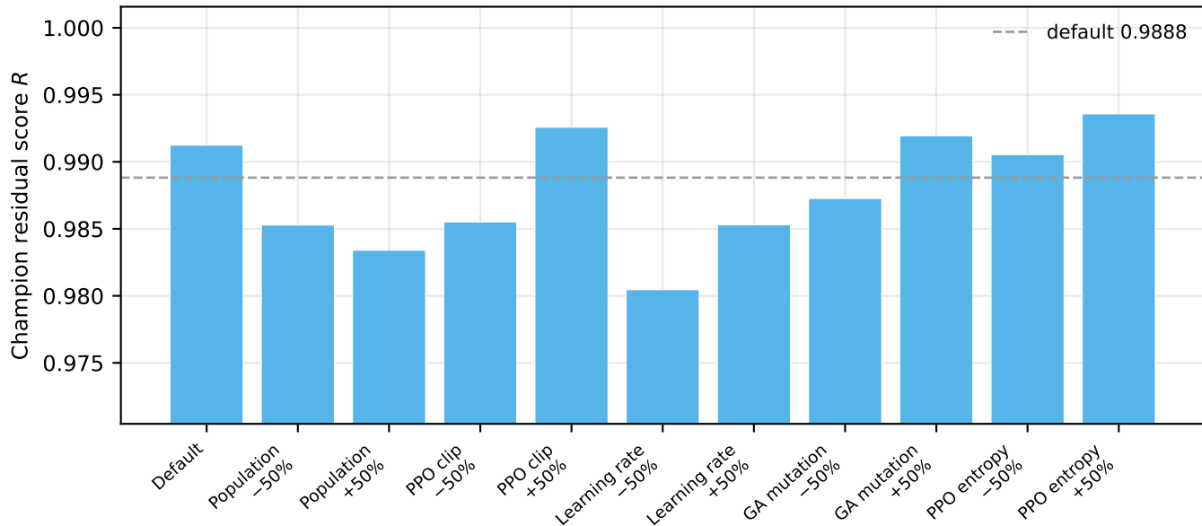
Sensitivity to 50% hyperparameter changes
