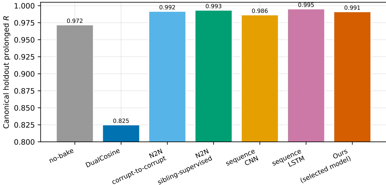
Noise2Noise and sequence baselines on the canonical holdout
