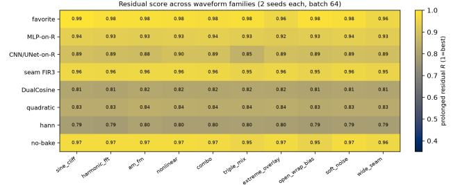
Figure 6: Colorblind-safe (cividis) heatmap of mean prolonged R for selected methods \times generative families (2 seeds each). Higher is better.
