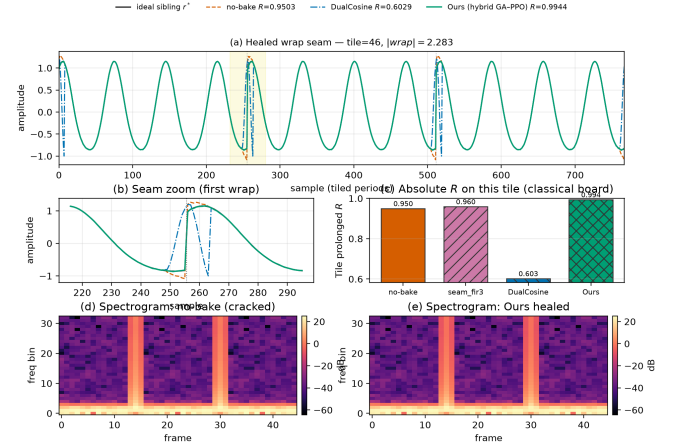
Figure 7: Holdout wrap-seam heal for the hybrid champion vs no-bake, Dual Cosine, and ideal sibling r^* (seed 20260719).
