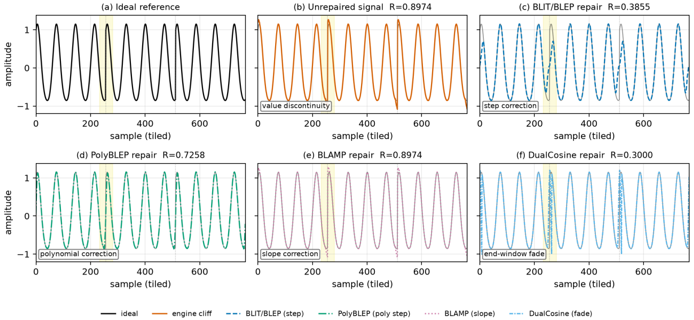
Figure 12: Classical VA seam techniques on one cracked sine+cliff tile (seed 20260719, tile 46, |wrap|=2.283 , L=256 , three tiled periods). Yellow band marks the first seam neighborhood. Panel tile R_{blend} (1 = best): (a) ideal (unscored sibling). (b) cracked engine 0.897. (c) BLIT/BLEP 0.385. (d) PolyBLEP 0.726. (e) BLAMP 0.897 (near no-bake on value cliffs). (f) DualCosine 0.300. Colorblind-safe hues with distinct linestyles for B&W print. Batch means appear in Table 14. Accessibility: six-panel comparison of ideal, cracked, BLIT/BLEP, PolyBLEP, BLAMP, and DualCosine.
