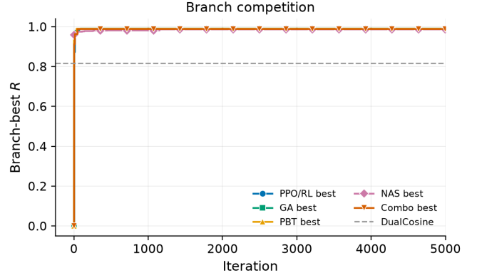
Figure 9: Overnight 5k-gate freeze: per-branch best residual trajectories (PPO/RL, GA, PBT, NAS, combo) versus iteration (x-axis capped at 5,000). Accessibility: colorblind-safe colors plus distinct markers (circle, square, triangle, diamond, inverted triangle) for grayscale print.
