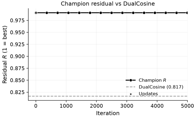
Figure 8: Overnight 5k-gate freeze: champion residual R versus clean search iteration (x-axis capped at 5,000), with DualCosine baseline on the runner geometry (RTX 3090). Accessibility: black line with circle markers; DualCosine as a dashed grey baseline.
