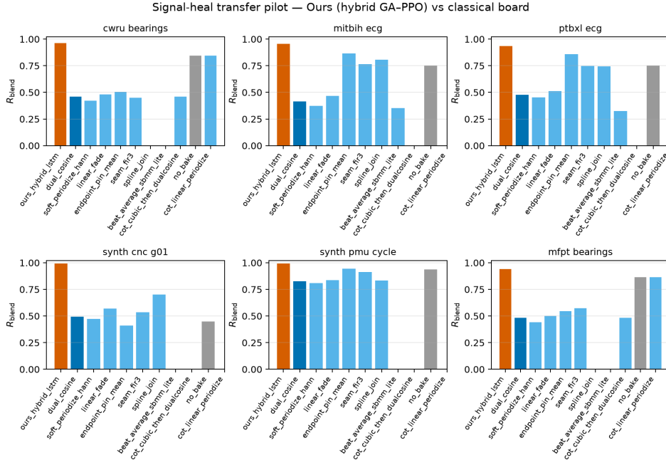
Figure 25: Transfer classical-board summary (holdout-refit R_{blend} ; grouped bars for Table 16). Not a deep-SOTA claim; see Table 17.
