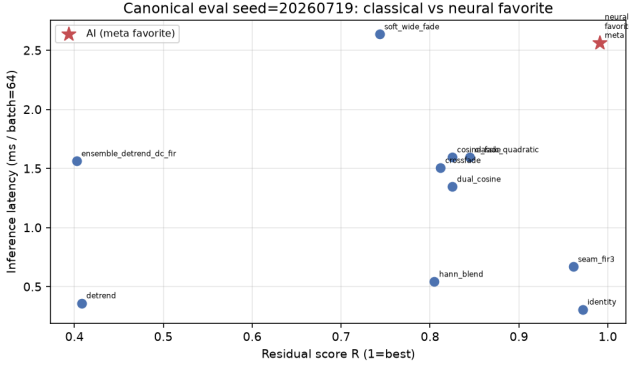
Figure 15: Canonical holdout (seed 20260719, batch 64): classical bake methods and neural favorite in the R vs CUDA ms/batch plane. Star: favorite.
