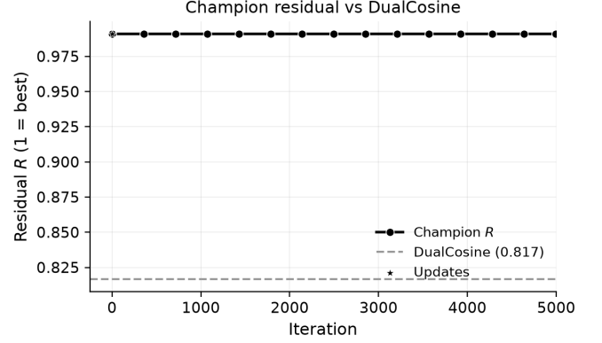
Figure 17: Champion residual R over the first 5,000 search iterations, with the DualCosine reference on the same runner geometry (RTX 3090). The black line uses circle markers; the reference is dashed gray.
