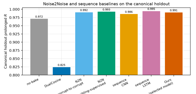
Figure 8: Canonical holdout prolonged R : N2N and seq baselines vs Ours (neural favorite). Train seeds 424242/424243 are disjoint from holdout 20260719.
