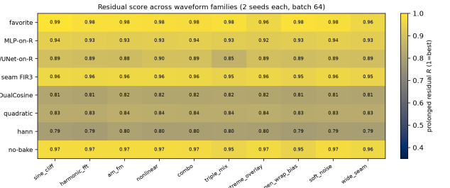
Figure 6: Colorblind-safe (cividis) heatmap of mean prolonged R for selected methods \times generative families (2 seeds each). Higher is better.
