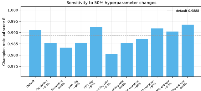
Figure 27: One-at-a-time \pm 50\% hyperparameter sensitivity of the hybrid champion residual R at a 500-iteration budget (seed 1902771841). The blue bar and dashed line mark the Table 2 default. This is a sensitivity probe, not a full 5,000-iteration search for each parameter.
