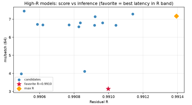
Figure 5: High- R fitted cells on CUDA (batch 64): prolonged residual R versus forward latency (ms/batch). Star marks the favorite (fastest inside the near-max- R band).
