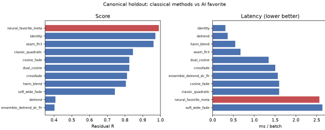
Figure 8: Canonical holdout ranking on prolonged residual R (left) and CUDA latency (right). DualCosine R \approx 0.825 . Favorite highlighted.
