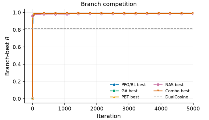
Figure 10: 5k-gate search freeze: per-branch best residual trajectories (PPO/RL, GA, PBT, NAS, combo) versus iteration (x-axis capped at 5,000). Accessibility: colorblind-safe colors plus distinct markers (circle, square, triangle, diamond, inverted triangle) for grayscale print.
