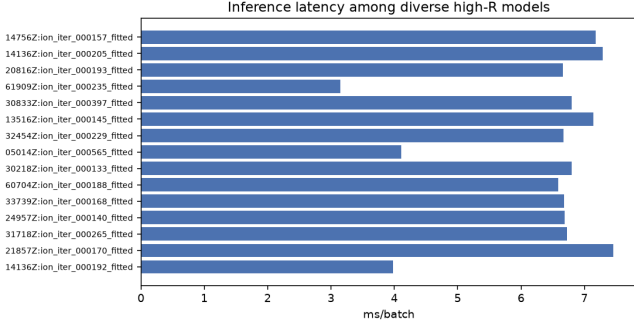
Figure 6: Inference latency (ms/batch, CUDA, batch 64) for diverse high- R fitted models from the inference bench.
