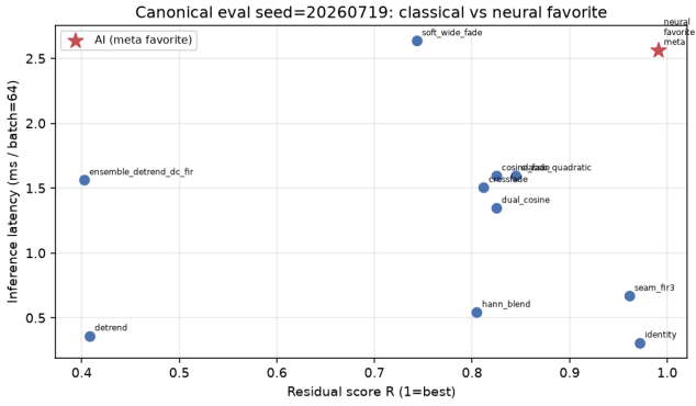
Figure 7: Canonical holdout (seed 20260719, batch 64): classical bake methods and neural favorite in the R vs CUDA ms/batch plane. Star: favorite.
