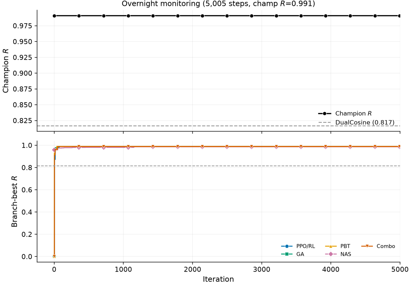
Figure 11: Full-width search monitoring panel at the 5k-gate freeze (first 5,000 iterations): champion R (top) and branch-best trajectories (bottom). Markers and Okabe-Ito colors match Figure 10. Source: history.jsonl .
