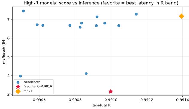
Figure 11: High- R fitted operators: residual vs CUDA latency. Star: favorite.
