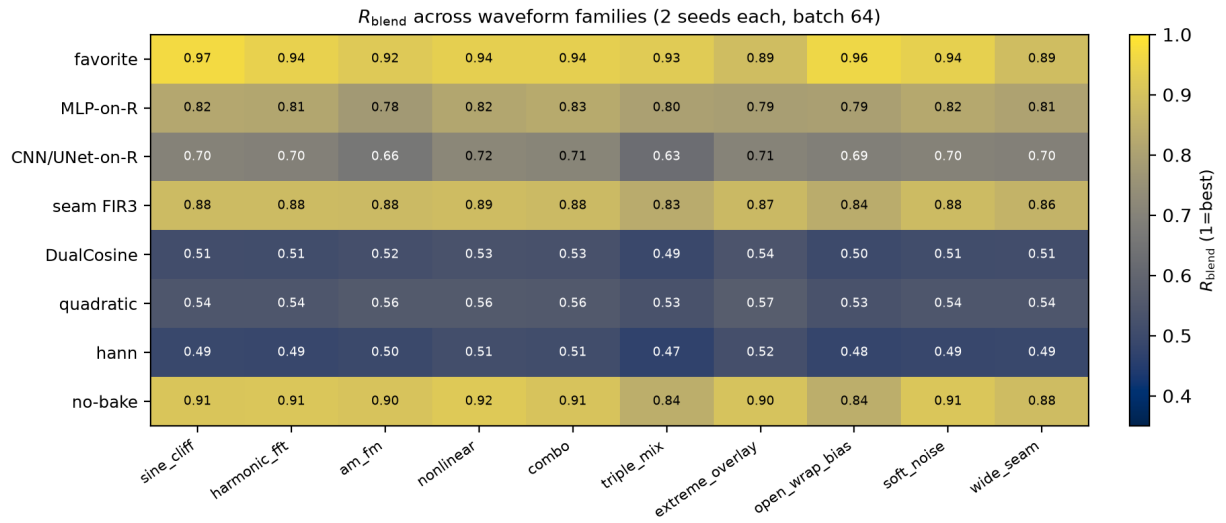
Figure 21: Colorblind-safe (cividis) heatmap of mean R_{\text{blend}} for selected methods \times generative families (2 seeds each). Higher is better.
