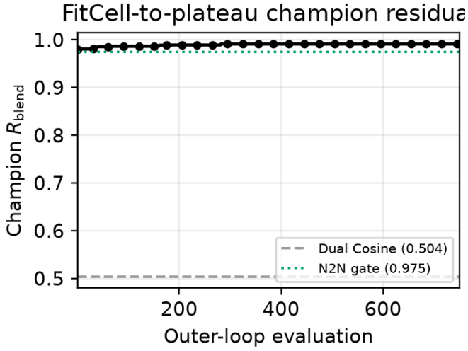
Figure 26: FitCell-to-plateau champion R_{\text{blend}} vs. outer-loop evaluation (seed 1902771841; Dual Cosine and Noise2Noise gate marked).
