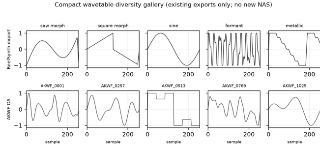
Figure 18: Compact wavetable diversity gallery from existing exports (one mid-morph dry frame per unique ReelSynth factory bank, top, and matched AKWF CC0 cycles, bottom). No new NAS for this panel. Quantitative wrap scores: Table 13.
