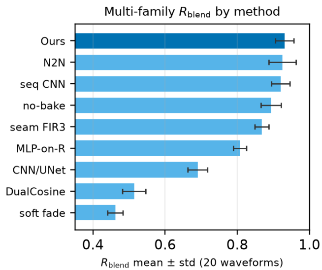
Figure 20: Multi-family mean R_{\text{blend}} by method (same 20-waveform board as Table 10).
