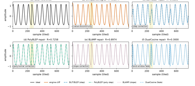
Figure 11: Classical VA seam techniques on one cracked sine+cliff tile (seed 20260719, tile 46). (a) ideal; (b) cracked engine; (c) BLIT/BLEP; (d) PolyBLEP; (e) BLAMP; (f) DualCosine. Batch means: Table 14.
