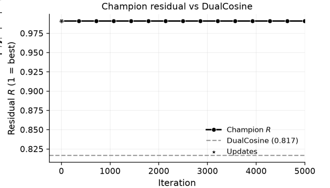
Figure 8: 5k-gate search freeze: champion residual R versus clean search iteration (x-axis capped at 5,000), with DualCosine baseline on the runner geometry (RTX 3090). Accessibility: black line with circle markers; DualCosine as a dashed gray baseline.
