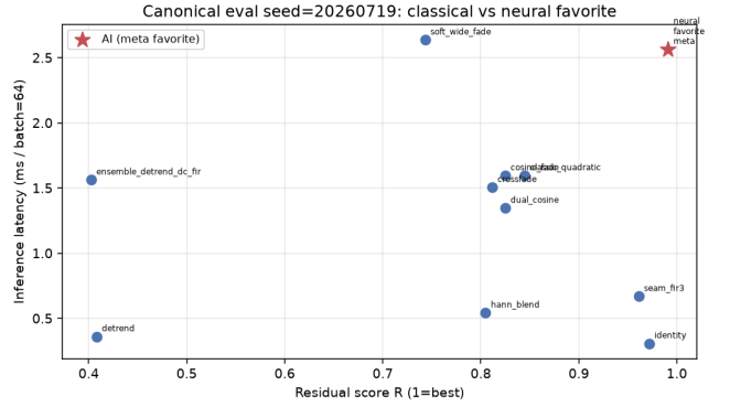
Figure 6: Canonical holdout (seed 20260719, batch 64): classical bake methods and neural favorite in the R vs CUDA ms/batch plane. Star: favorite.
