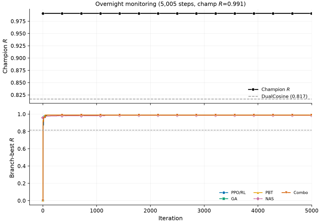
Figure 10: Full-width search monitoring panel at the 5k-gate freeze (first 5,000 iterations): champion R (top) and branch-best trajectories (bottom). Markers and Okabe-Ito colors match Figure 9. Source: history.jsonl .
