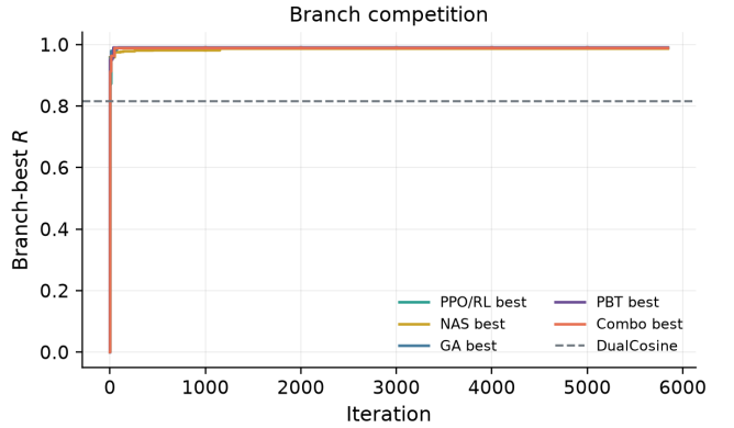
Figure 9: Overnight 5k-gate freeze: per-branch best residual trajectories (PPO/RL, GA, PBT, NAS, combo) versus iteration. Accessibility: multi-series line plot; branches distinguished by color (shape markers deferred).
