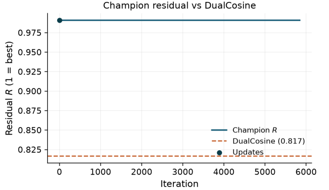
Figure 8: Overnight 5k-gate freeze: champion residual R versus clean search iteration, with DualCosine baseline on the runner geometry (RTX 3090). Accessibility: line plot of champion R over iterations.
