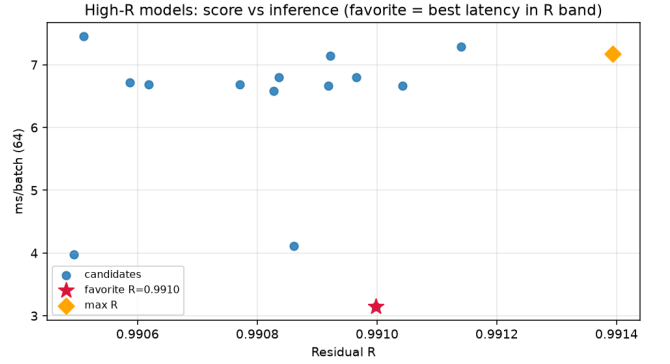
Figure 4: High- R fitted cells on CUDA (batch 64): prolonged residual R versus forward latency (ms/batch). Star marks the favorite (fastest inside the near-max- R band).
