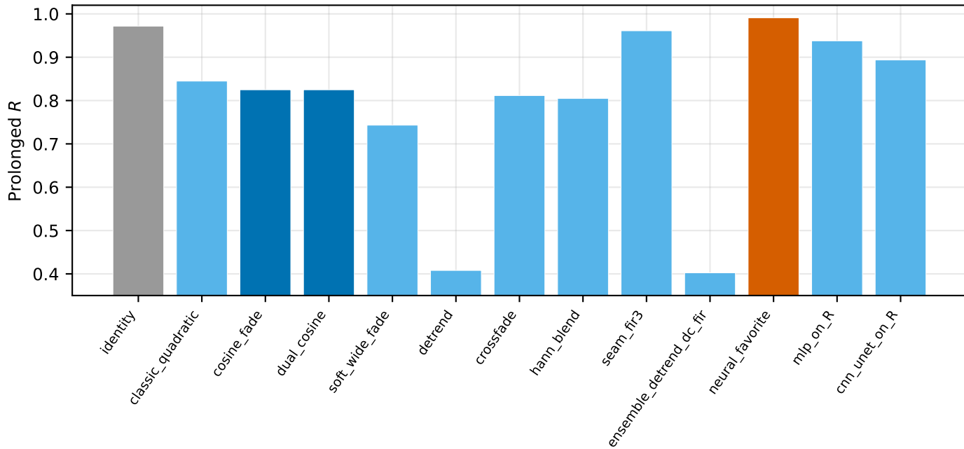
Canonical holdout: classical vs AI methods
