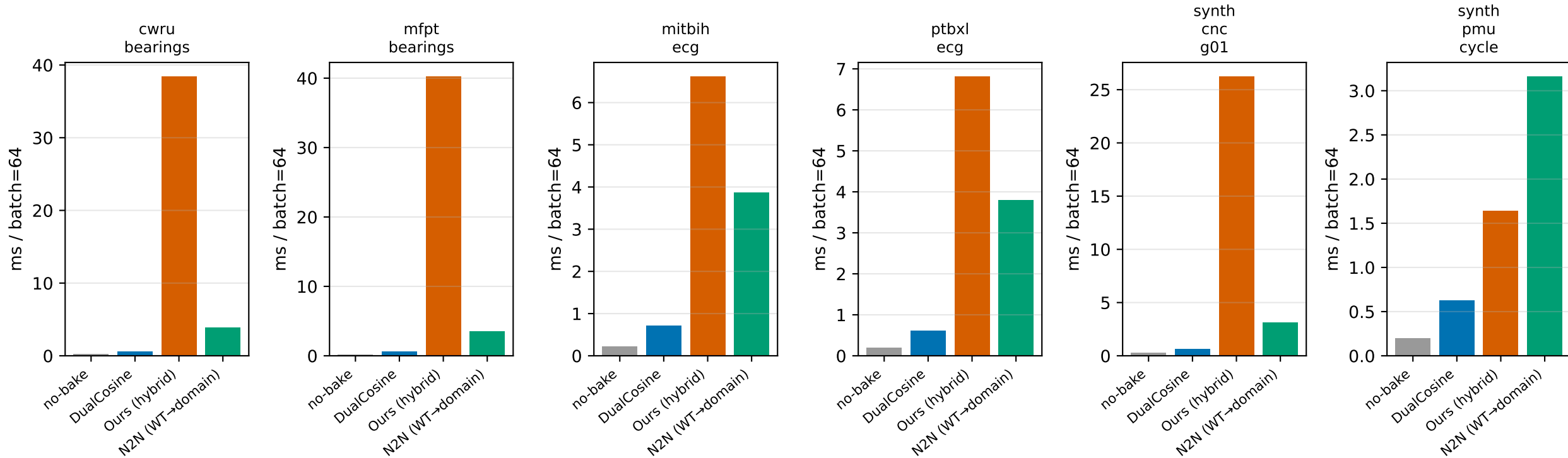
Transfer-domain inference latency (device in JSON; warmup/timed fixed)
