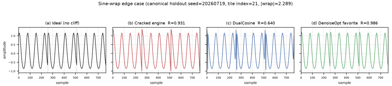
Figure 1: Sine-wrap edge case from the canonical eval holdout (same tile). Ideal periodic reference, cracked engine with wrap seams (dashed), DualCosine bake, and DenoiseOpt favorite. Prolonged residual R is printed per panel.
