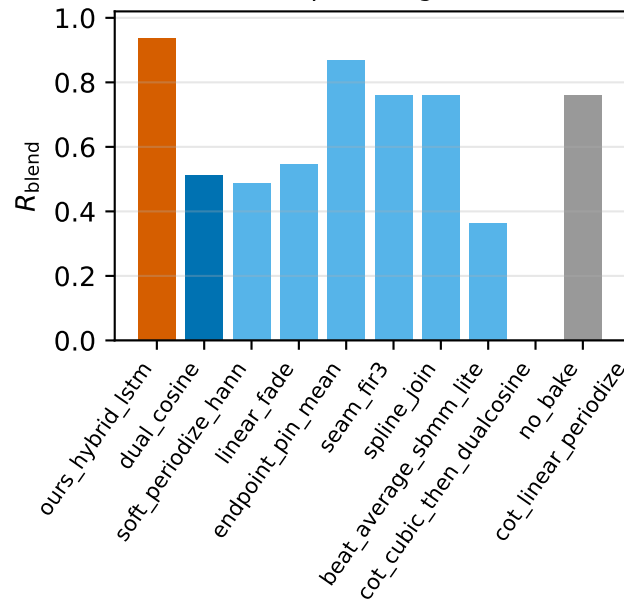
mfpt bearings
