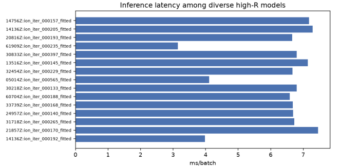
Figure 3: Inference latency (ms/batch, CUDA, batch 64) for diverse high- R fitted models from the inference bench.
